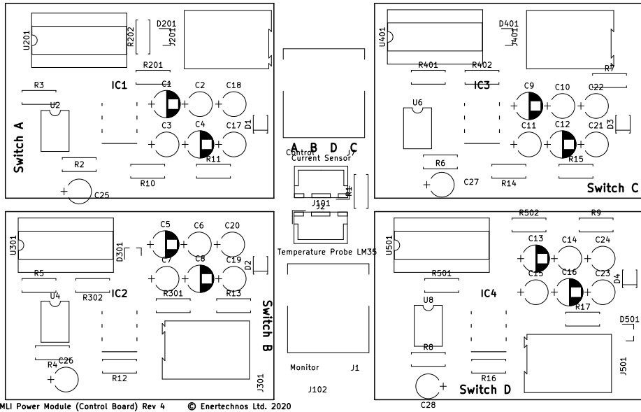
MLI Power Module (Control Board) Rev 4 © Enertechnos Ltd. 2020
